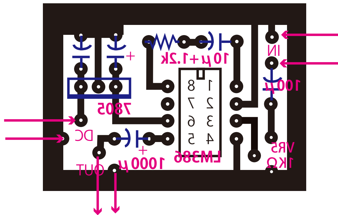
Gain50 AMP+DC5V
